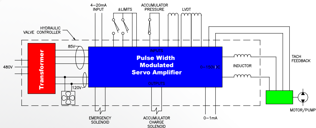
Valve Controller System Schematic
